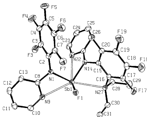
Figure 1. Molecular structure of 7 ; hydrogen atoms and solvate toluene molecule are omitted for clarity
